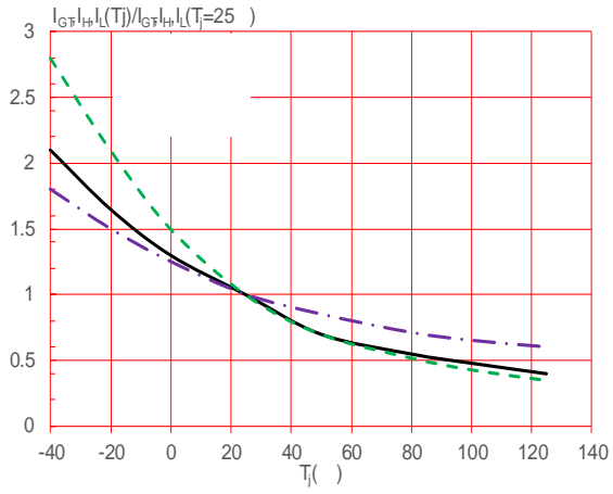
FIG.7: R_{th(j-c)} \mu m
