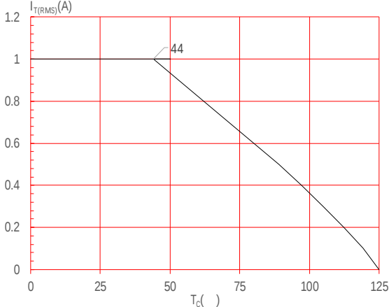
FIG.4: On-state characteristic
